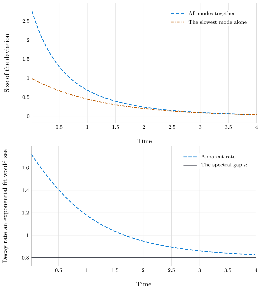
Figure 14.3: Above: a deviation from stationarity with positive weight on four modes, against the slowest mode alone. The total starts above the slowest mode and approaches it from above, because the higher modes are still alive early and decaying faster. Below: the decay rate an exponential fit would report if it began at that time, against the spectral gap it is supposed to be estimating. Early windows see a rate well above \kappa and the bias is one-sided — which is the same overstatement of mean reversion chapter 20’s calculation. Where the bias comes from and what it scales with finds from the estimator’s side, arriving here from the spectrum’s.
